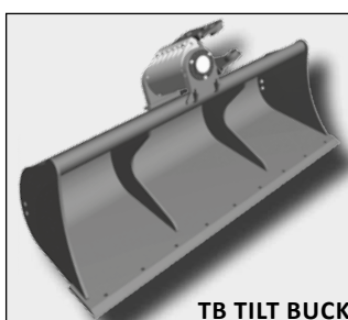
TB TILT BUCKET More flexibility and maneuverability due to a tilt angle of 140° up to 180°
